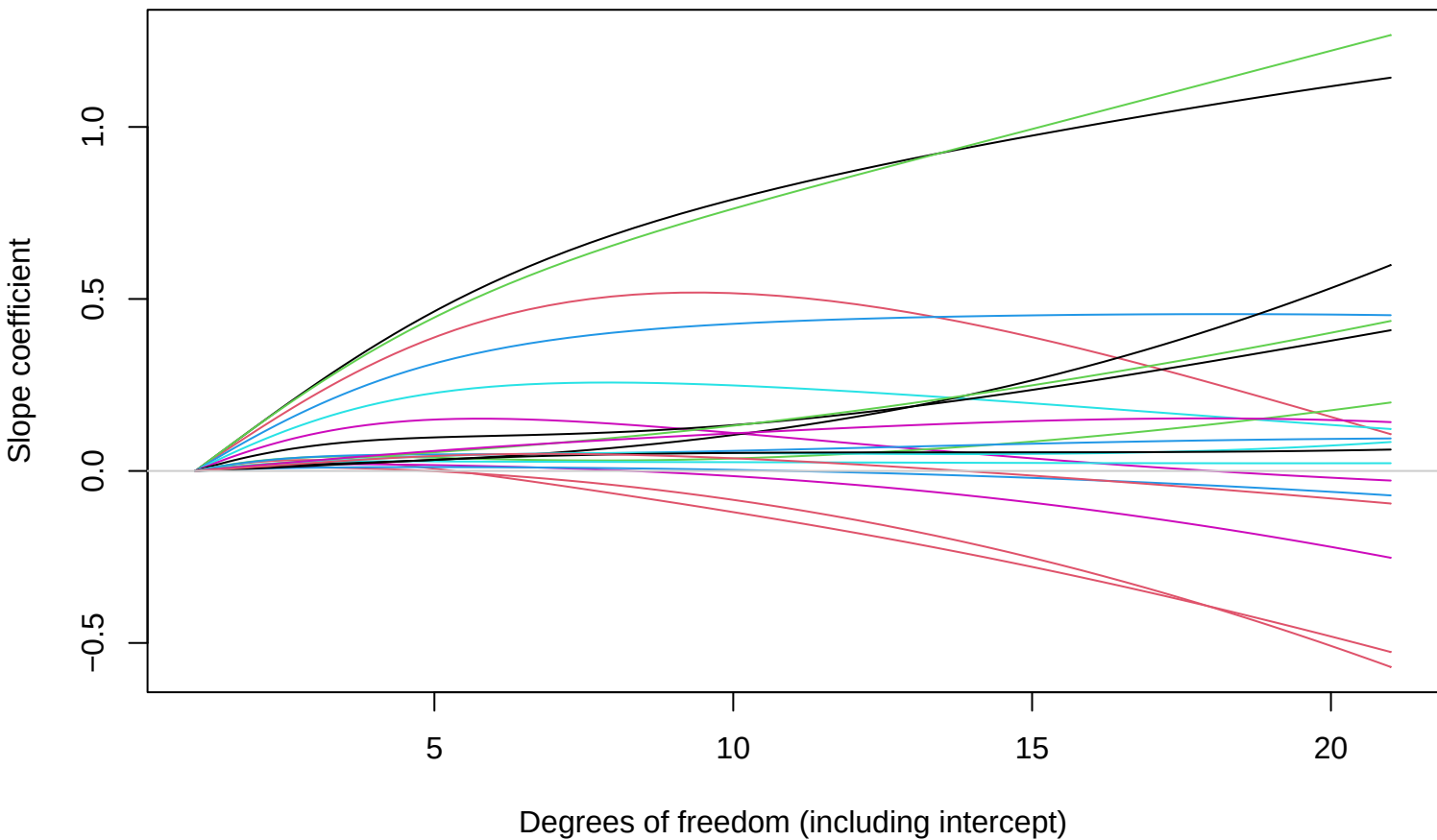
ridge coefficient path: p = 20
